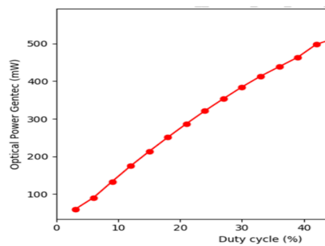
Average optical power of the laser as a function of the laser duty cycle with a pulswidth of 900ns and a laser temperature of +20^\circ\text{C}
