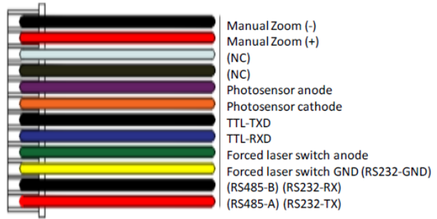
Connection of Control Line (12 PIN)
