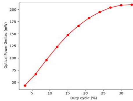
Average optical power of the laser as a function of the laser duty cycle with a pulsewidth of 900ns and a laser temperature of +20°C
